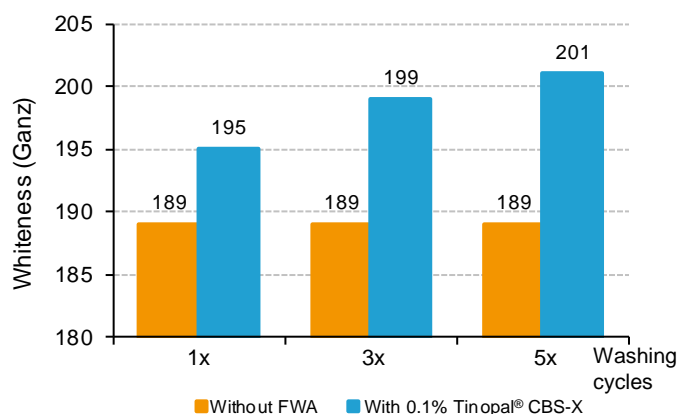
Improved whiteness due to Tinopal® CBS-X application in fabric (100% cotton pre-brightened)
