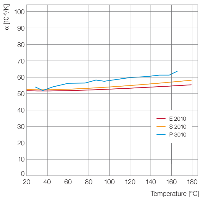
Fig. 24: Coefficient of linear thermal expansion according to DIN 53752
